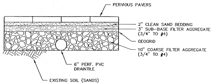
PERVIOUS PAVEMENT DETAIL
