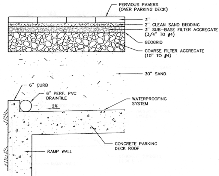
PERVIOUS PAVERS OVER UNDERGROUND PARKING STRUCTURE NO SCALE
