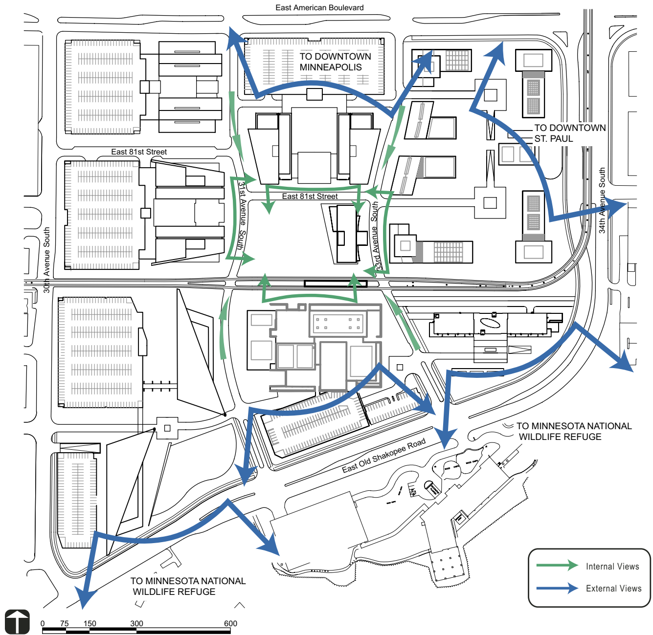
Figure 17: View Corridor Diagram
