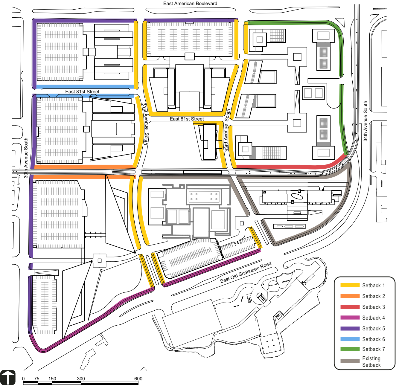
Figure 20: Setback Diagram
