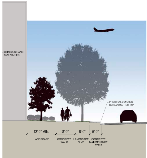
Figure 27a: Zone IVB Perimeter: Streetscape Plan
