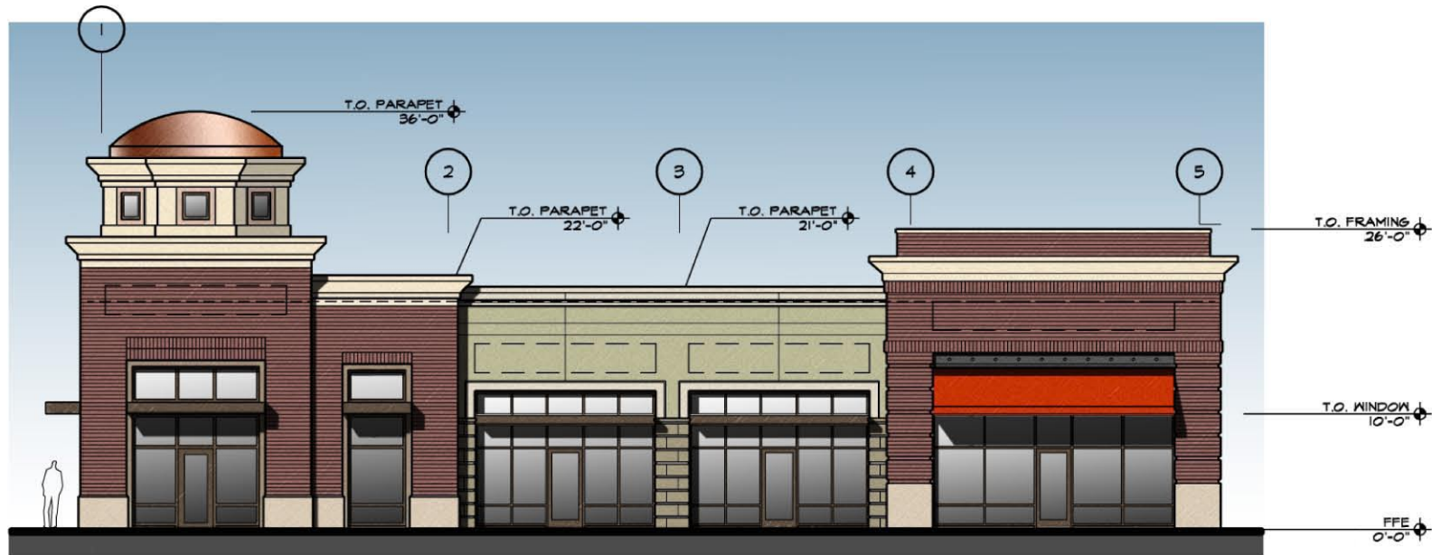
1 NORTH ELEVATION A202 1/16" = 1'-0"
